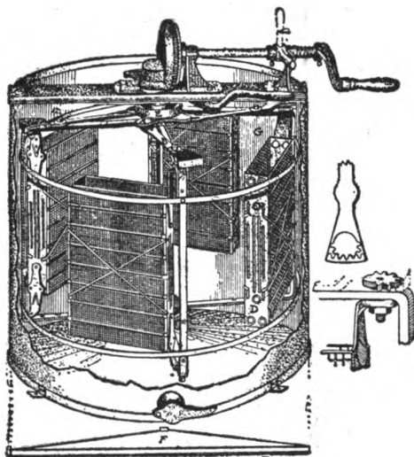
Fig. 43.—“AUTOMATIC” FOUR-COMB REVERSIBLE EXTRACTOR.
