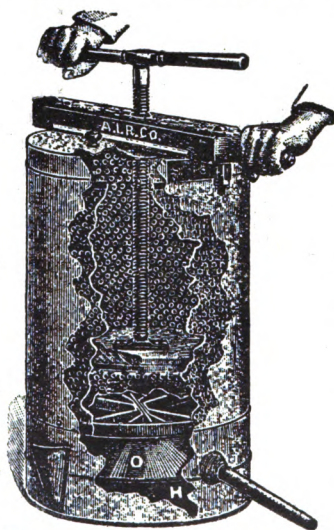
Fig. 12.—GERMAN STEAM WAX PRESS.
