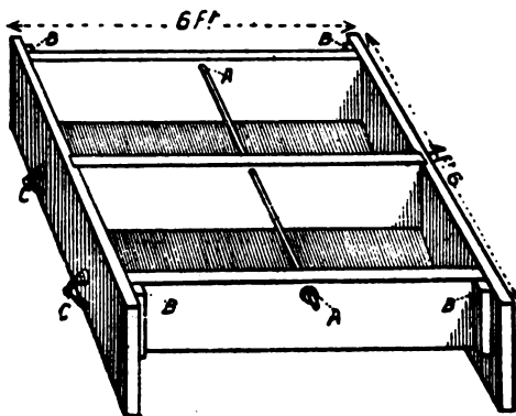
Fig. 76.—HONEY TANK. (Not drawn to scale.)
