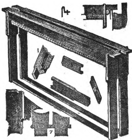
Fig. 32.—THE HOFFMAN BROOD AND EXTRACTING FRAMES.
